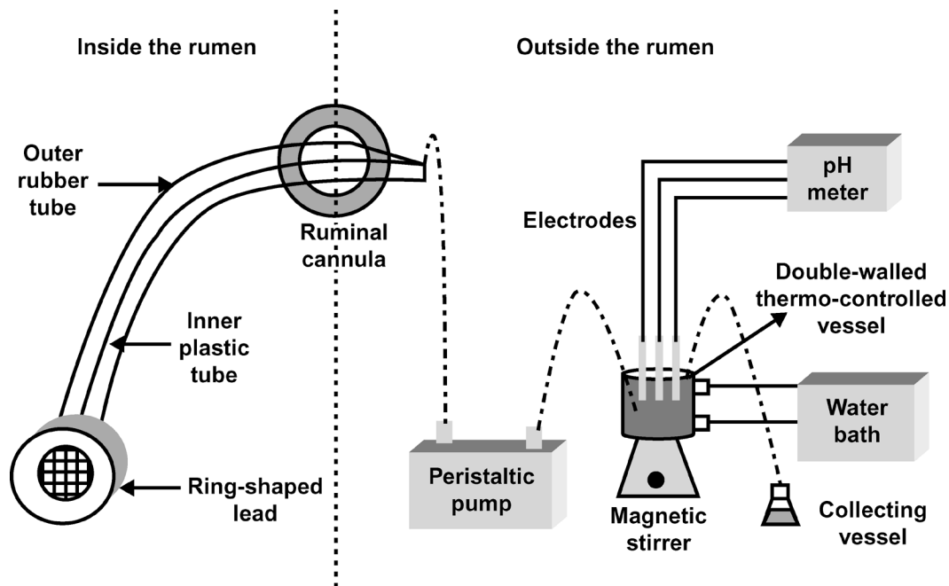
Figure 1. Method of continuous sampling and measurements with elimination of gaseous contamination.
